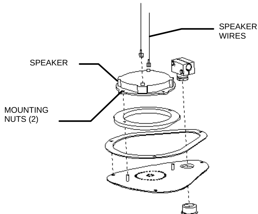
SPEAKER/MICROPHONE ASSEMBLY DETAIL ILLUSTRATION 1-2
