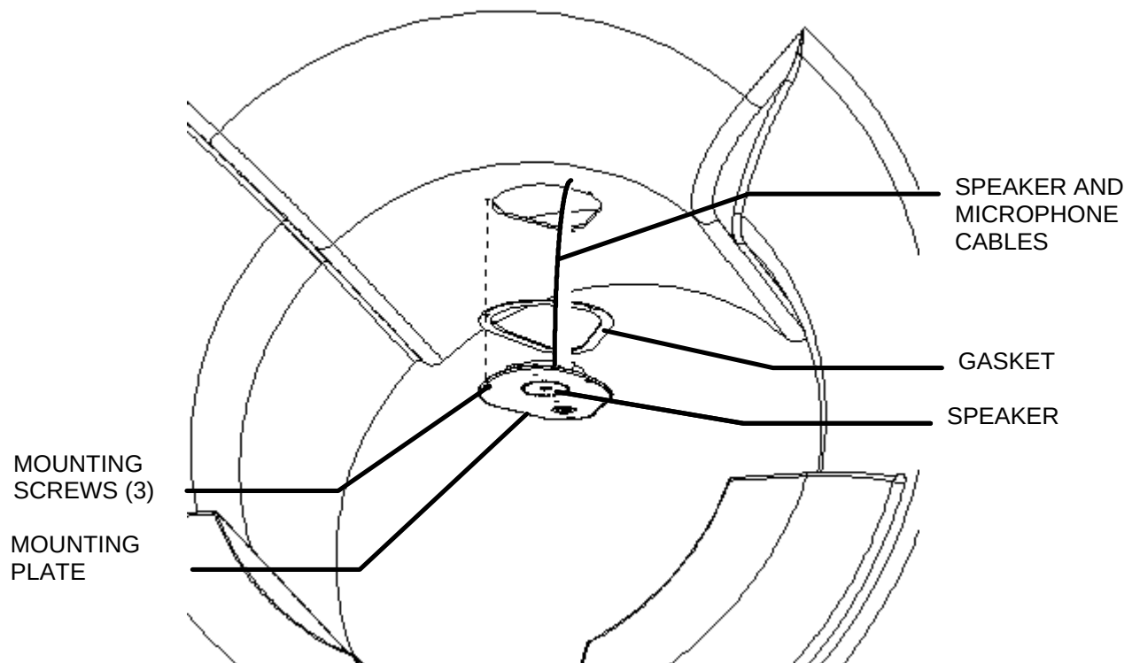
SPEAKER/MICROPHONE ASSEMBLY ILLUSTRATION 1-1
